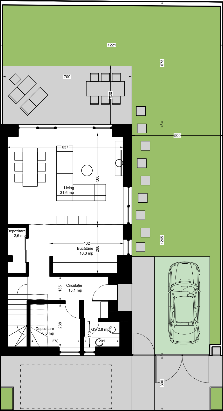
plan parter
