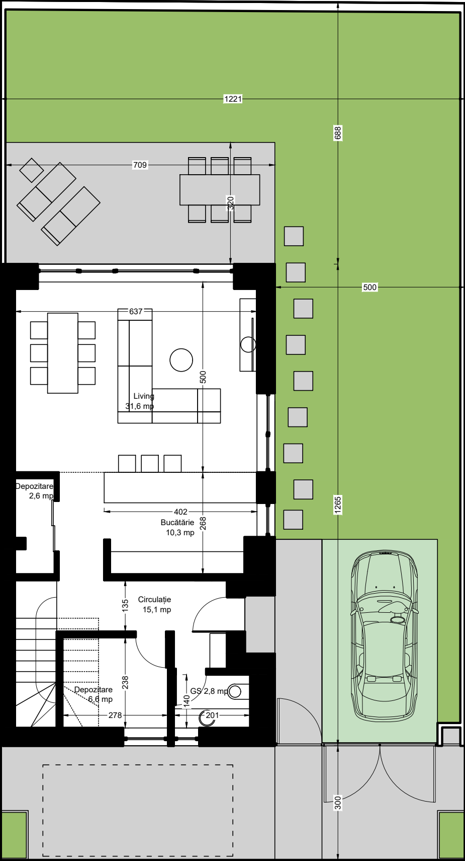
plan parter
