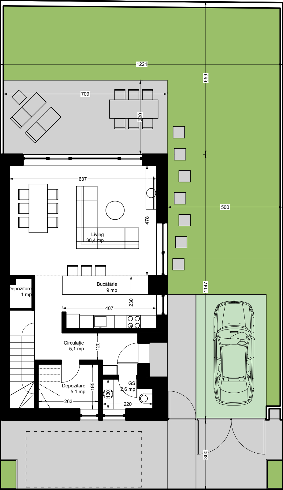
plan parter
