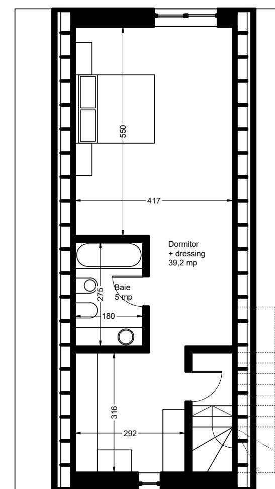
Plan mansardă
