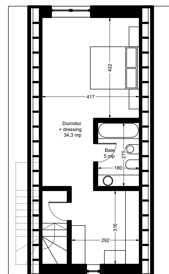
Plan mansardă
