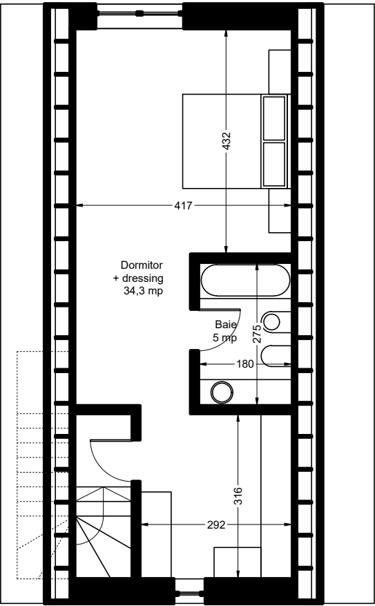
Plan mansardă
