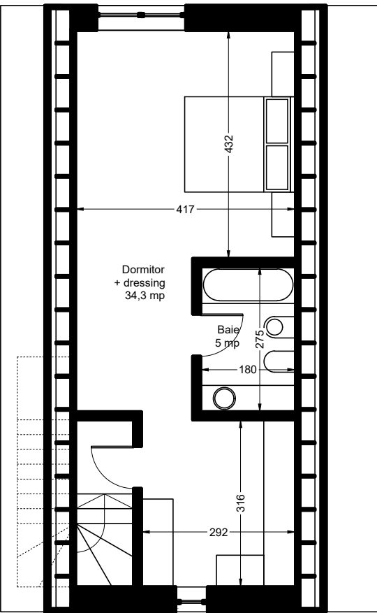
Plan mansardă
