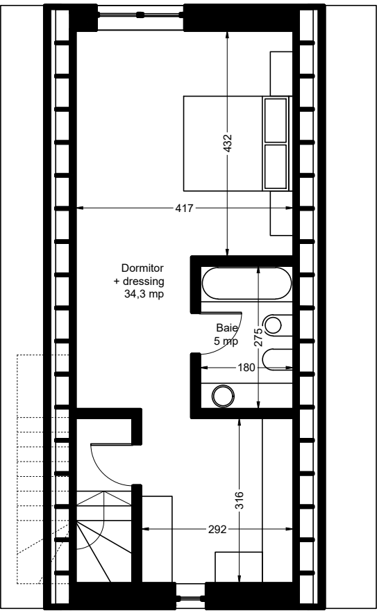
Plan mansardă
