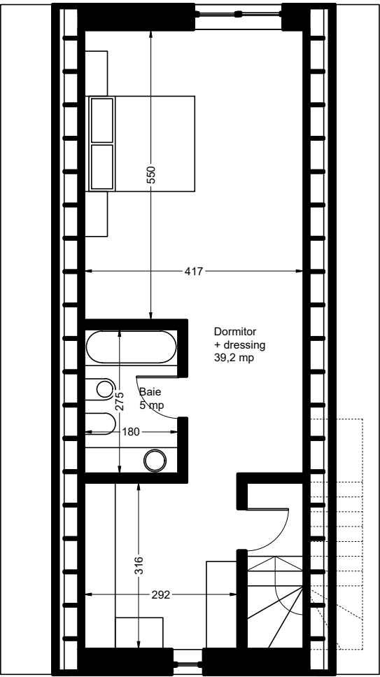
Plan mansardă
