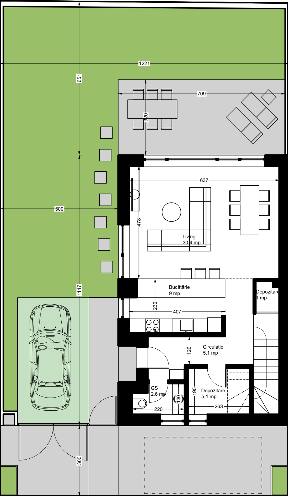
plan parter
